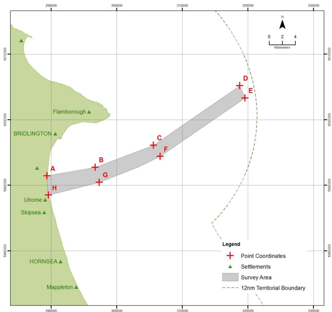
Figure 1: Above; survey area plan for near-shore geophysical survey activity – MV Ivero
